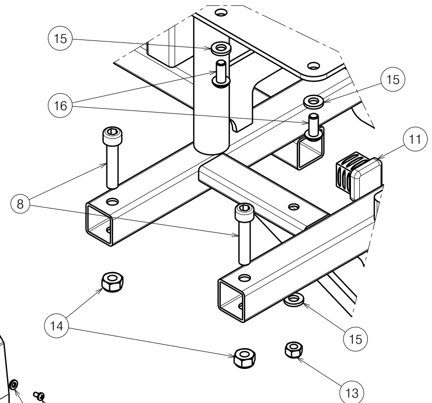
Detail View A (1:2)
